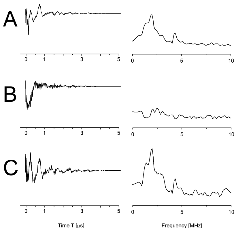
FIGURE 6: REFINE spectra of complex I at 17 K. For all experiments, a \tau value of 192 ns is used. All spectra are taken at a magnetic field corresponding to g = 1.96 and are normalized to the echo intensity at t = 0 . Panel A presents the REFINE spectrum with a 50 \mu\text{s} filter time. Panel B presents the REFINE spectrum with a filter time to suppress the contributions of cluster N1. No modulations are left. Panel C presents the REFINE with a filter time taken to suppress contributions of cluster N2.
